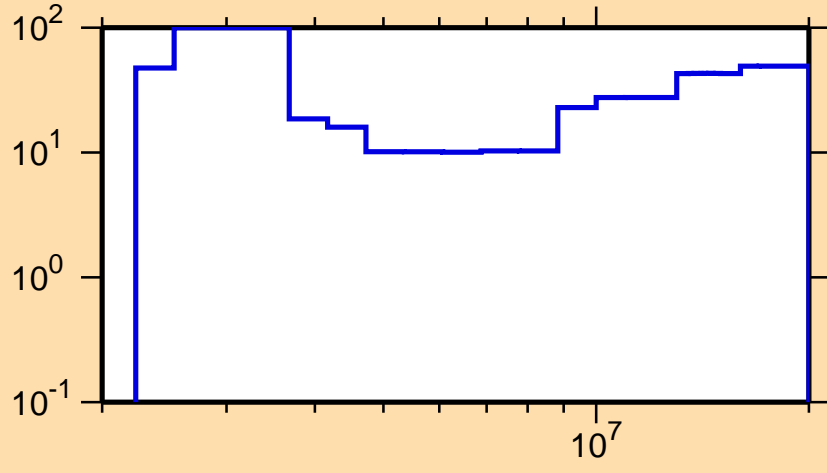
\Delta\sigma/\sigma vs. E for ^{86}\text{Y}(n,n\text{cont.})
