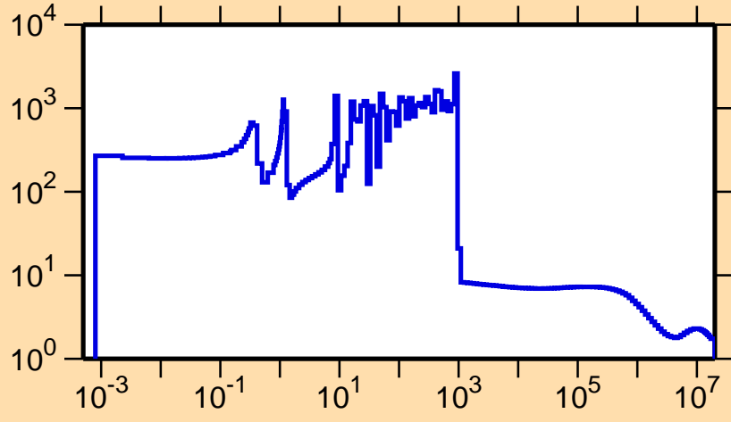
\sigma vs. E for ^{86}\text{Y}(n,\text{el.})
