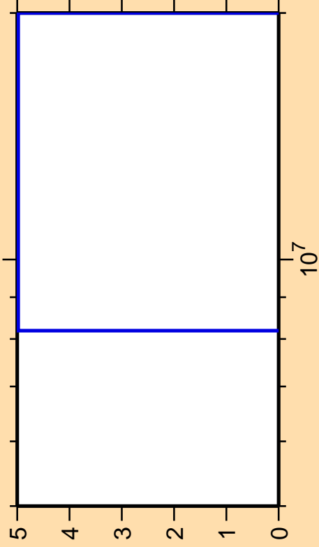
\Delta\sigma/\sigma vs. E for ^{86}\text{Y}(n,\text{pt})
