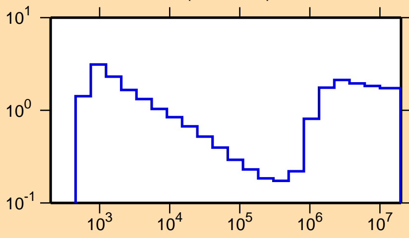
\sigma vs. E for ^{87}\text{Y}(n,\text{nonel.})
