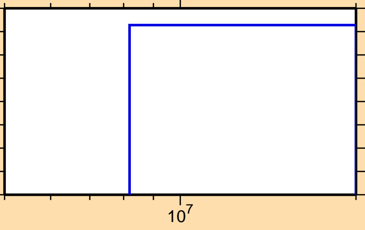
\sigma vs. E for ^{87}\text{Y}(n,\text{nd})
