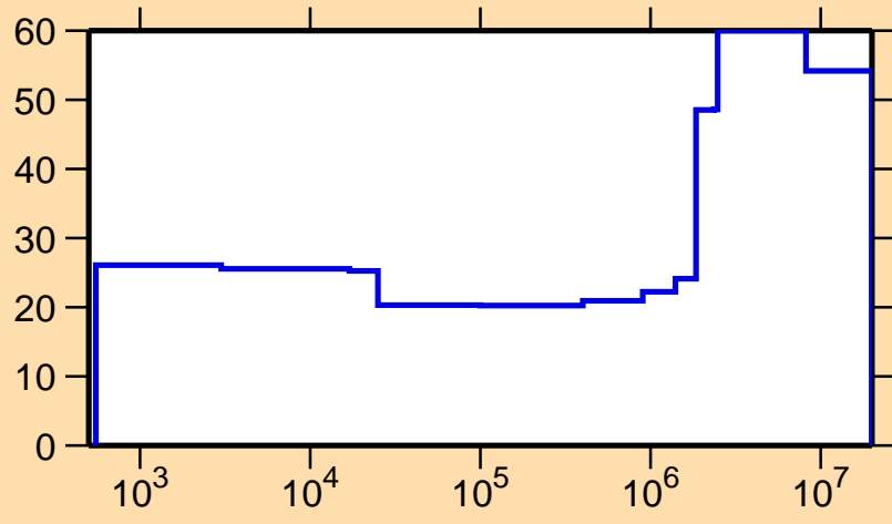
\Delta\sigma/\sigma vs. E for ^{87}\text{Y}(n,\gamma)
