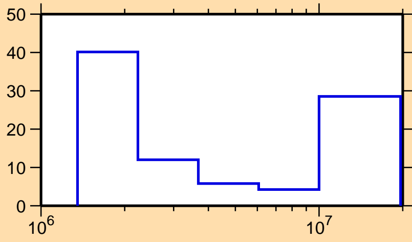
\Delta\sigma/\sigma vs. E for ^{87}\text{Y}(n,n\text{cont.})
