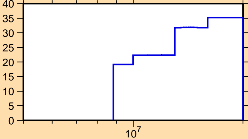
\Delta\sigma/\sigma vs. E for ^{88}\text{Y}(n,\text{inel.})
