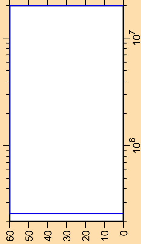
\Delta\sigma/\sigma vs. E for ^{88}\text{Y}(n,\alpha)
