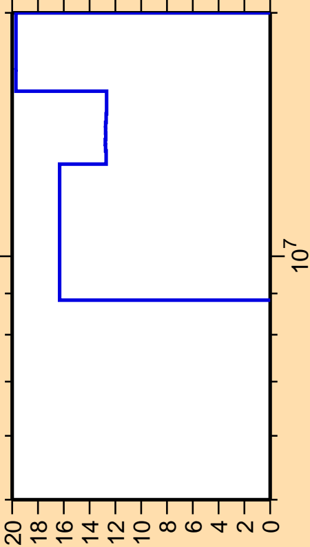
\Delta\sigma/\sigma vs. E for ^{88}\text{Y}(n,2n)
