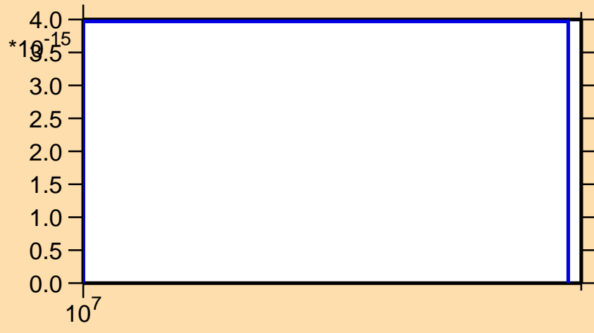
\sigma vs. E for ^{88}\text{Y}(n,\text{pd})
