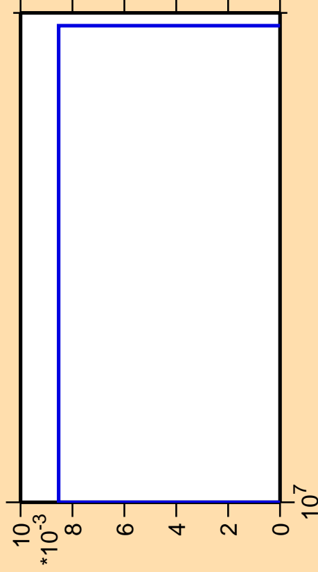
\Delta\sigma/\sigma vs. E for ^{88}\text{Y}(n,2n\alpha)
