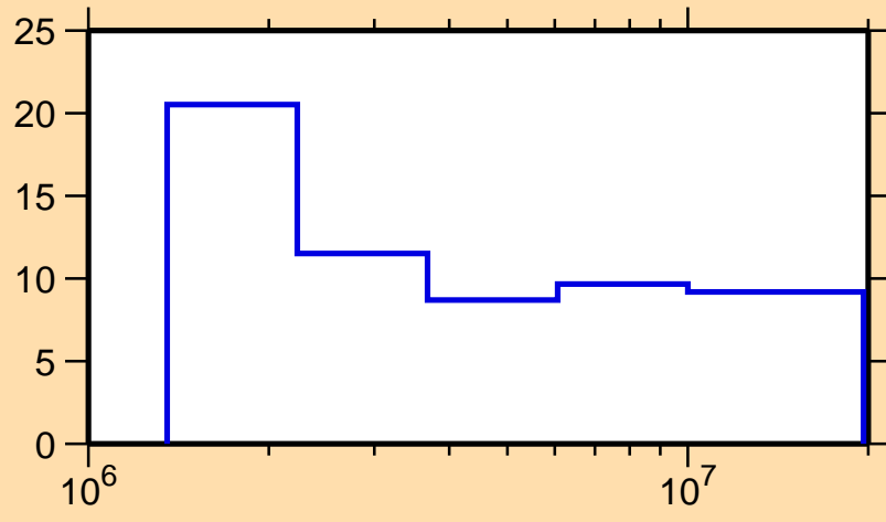
\Delta\sigma/\sigma vs. E for ^{88}\text{Y}(n,n\text{onel.})
