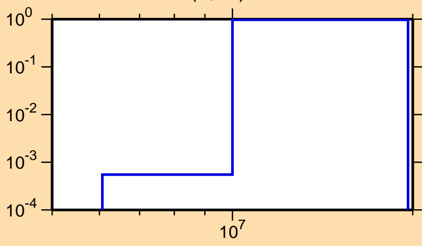
\sigma vs. E for ^{88}\text{Y}(n,2n)
