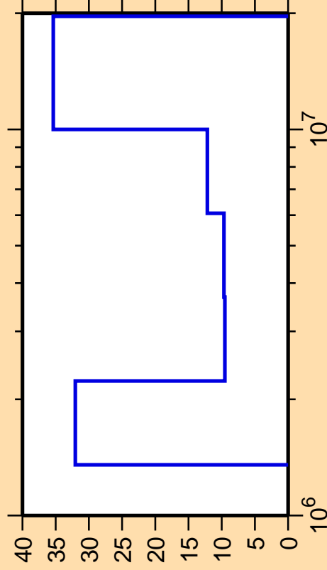
\Delta\sigma/\sigma vs. E for ^{88}\text{Y}(n,\text{ncont.})
