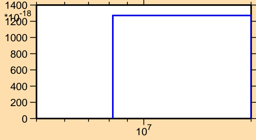
\sigma vs. E for ^{88}\text{Y}(n,2n\alpha)
