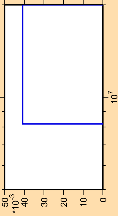
\Delta\sigma/\sigma vs. E for ^{88}\text{Y}(n,\text{pd})
