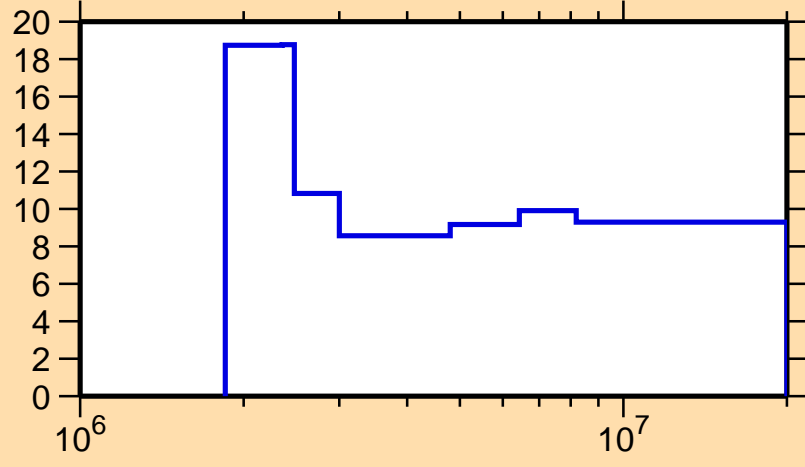
\Delta\sigma/\sigma vs. E for ^{88}\text{Y}(n,n_{\text{nonel}})
