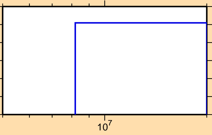
\sigma vs. E for ^{88}\text{Y}(n,\text{nd})
