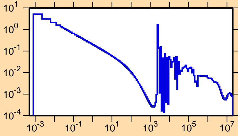
\sigma vs. E for ^{89}\text{Y}(n,\gamma)
