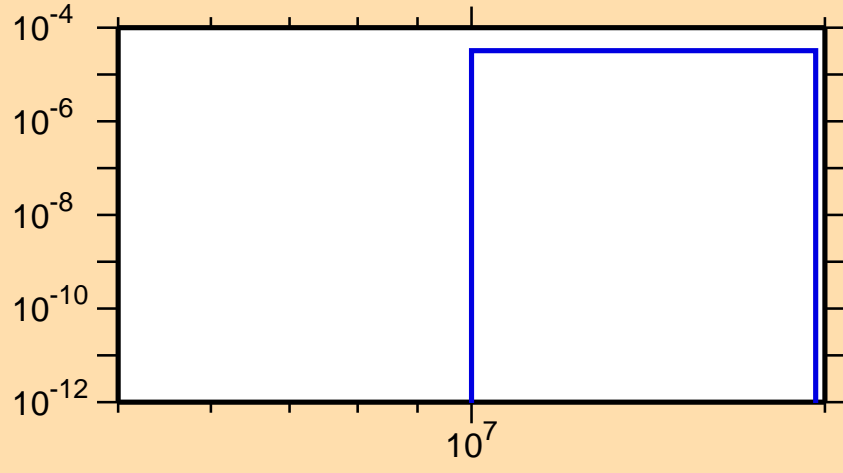
\sigma vs. E for ^{89}\text{Y}(n,n\alpha)
