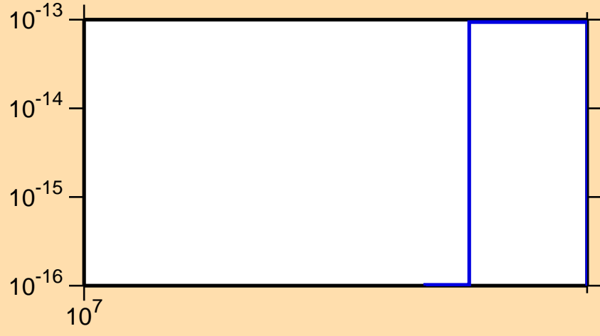
\sigma vs. E for ^{89}\text{Y}(n,\text{pd})
