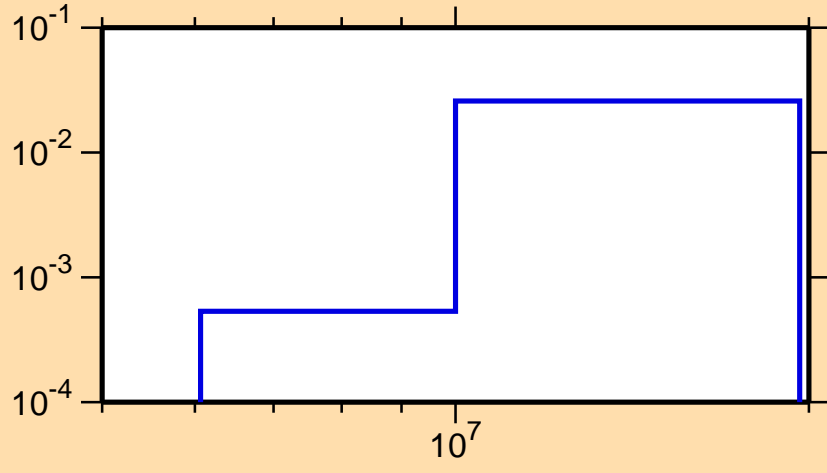
\sigma vs. E for ^{89}\text{Y}(n,np)
