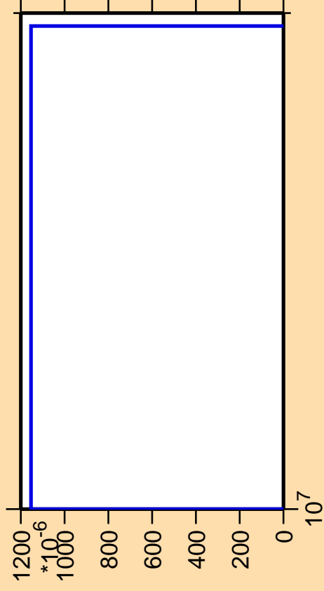
\Delta\sigma/\sigma vs. E for ^{89}\text{Y}(n,\text{pd})
