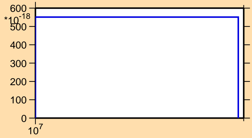
\sigma vs. E for ^{89}\text{Y}(n,\text{pd})
