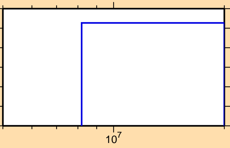
\sigma vs. E for ^{89}\text{Y}(n,n\alpha)
