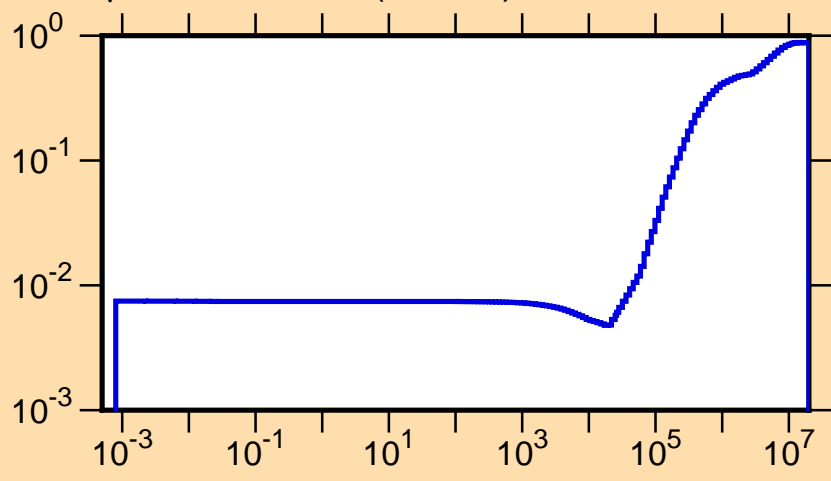
\mu vs. E for ^{90}\text{Y}(\text{mt251})
