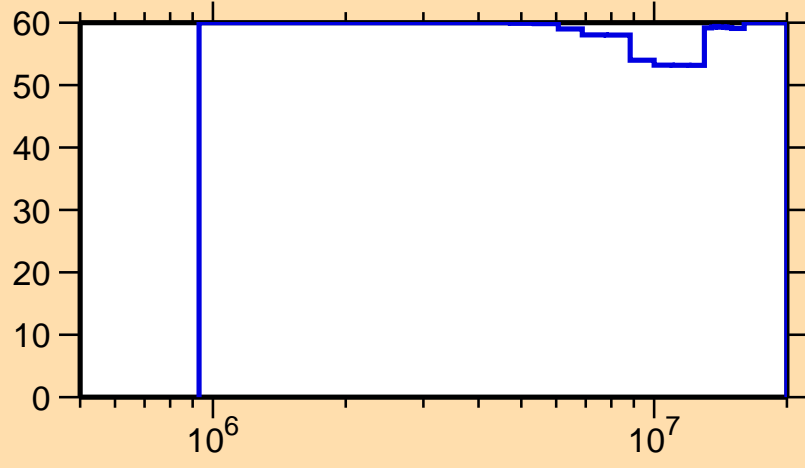
\Delta\sigma/\sigma vs. E for ^{90}\text{Y}(n,p)
