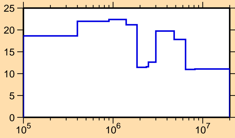
\Delta\sigma/\sigma vs. E for ^{90}\text{Y}(n,el.)
