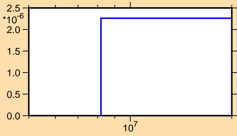
\sigma vs. E for ^{90}\text{Y}(n,\text{nd})
