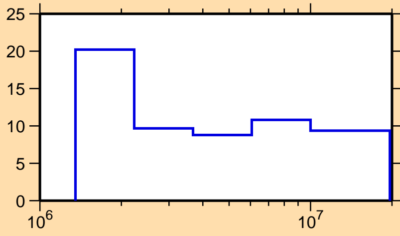
\Delta\sigma/\sigma vs. E for ^{90}\text{Y}(n,n\text{nonel.})
