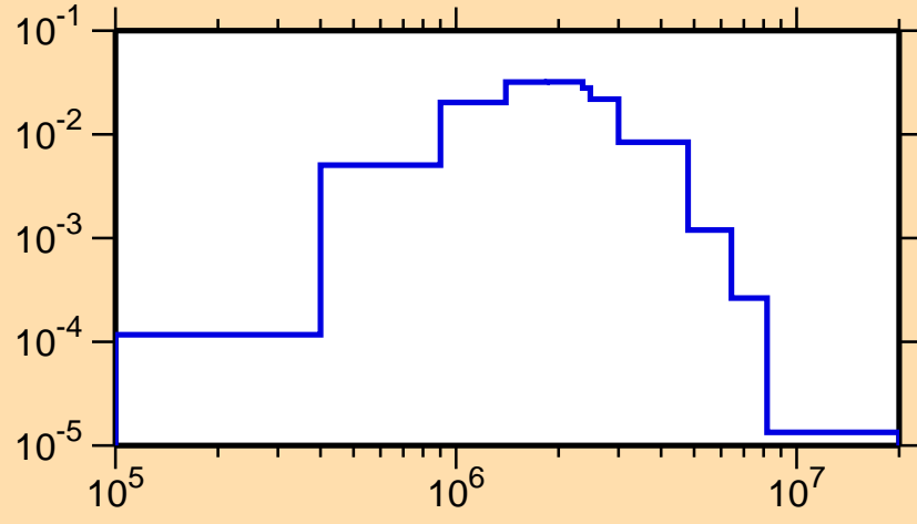
\sigma vs. E for ^{90}\text{Y}(n,n_4)
