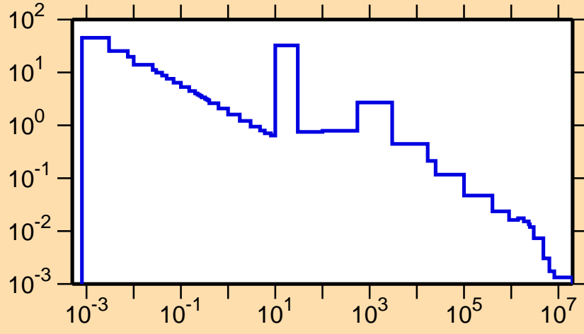
\sigma vs. E for ^{90}\text{Y}(n,\gamma)
