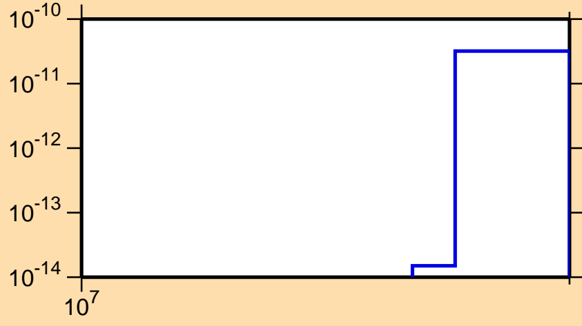
\sigma vs. E for ^{91}\text{Y}(n,\text{He}3)
