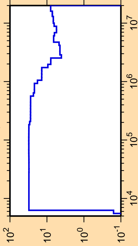
\Delta\sigma/\sigma vs. E for ^{91}\text{Y}(n,\text{nonel.})
