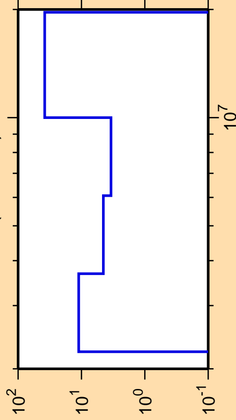
\Delta\sigma/\sigma vs. E for ^{91}\text{Y}(n,\text{ncont.})
