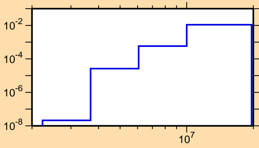
\sigma vs. E for ^{91}\text{Y}(n,p)
