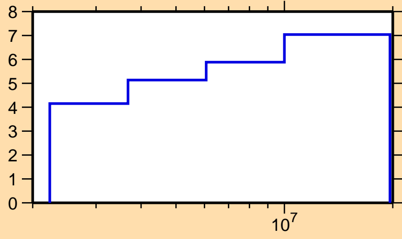
\Delta\sigma/\sigma vs. E for ^{91}\text{Y}(n,n\text{onel.})
