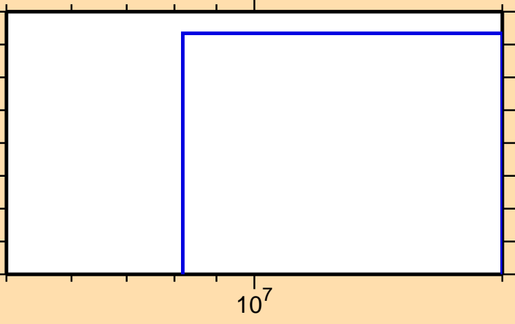
\sigma vs. E for ^{91}\text{Y}(n,nt)
