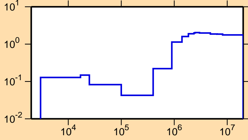
\sigma vs. E for ^{91}\text{Y}(n,\text{nonel.})
