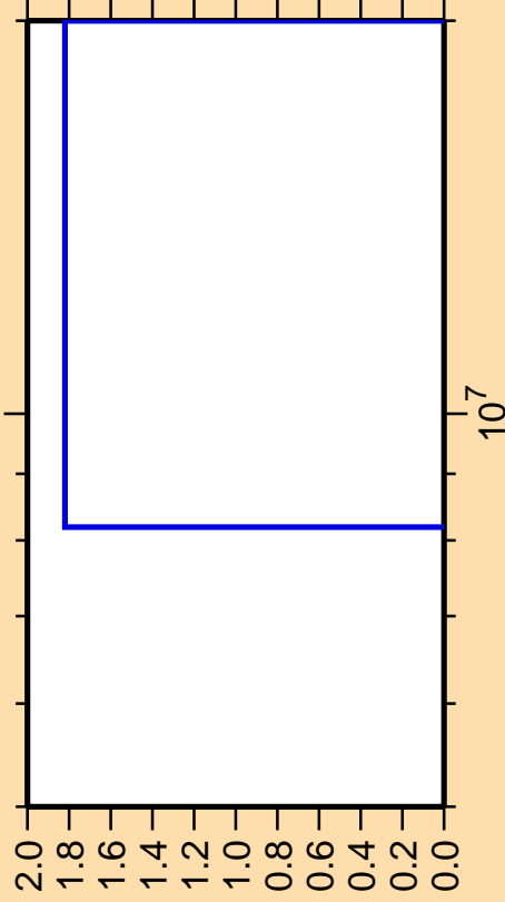
\Delta\sigma/\sigma vs. E for ^{91}\text{Y}(n,\text{He}3)
