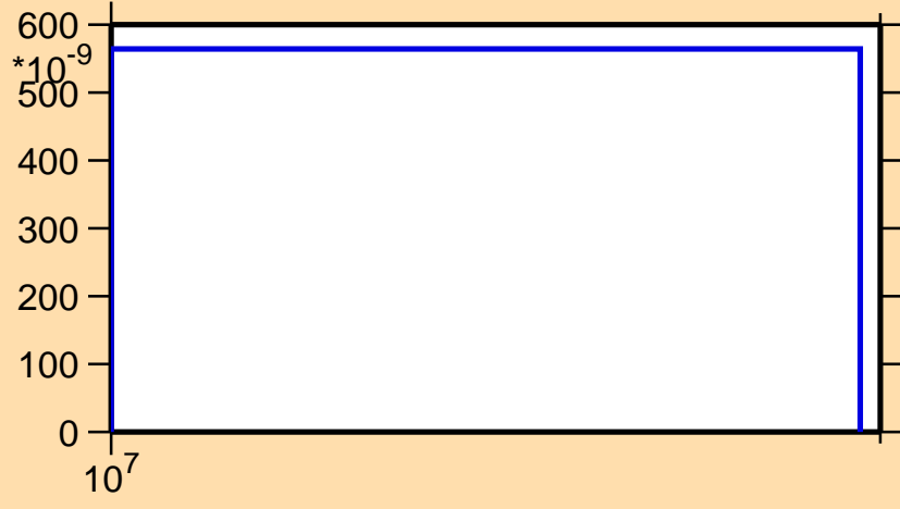
\sigma vs. E for ^{91}\text{Y}(n,\text{nd})
