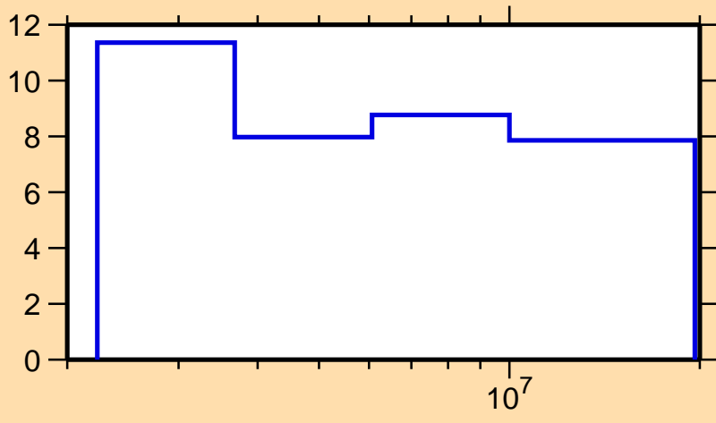
\Delta\sigma/\sigma vs. E for ^{91}\text{Y}(n,n\text{onel.})
