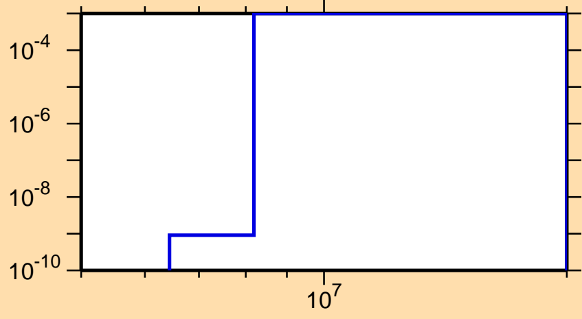
\sigma vs. E for ^{91}\text{Y}(n,d)
