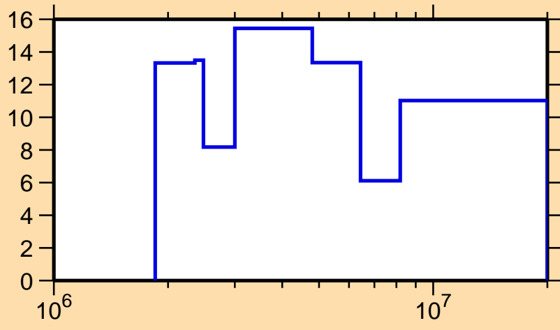
Δσ/σ vs. E for ^{91}\text{Y}(n,\text{el.})
