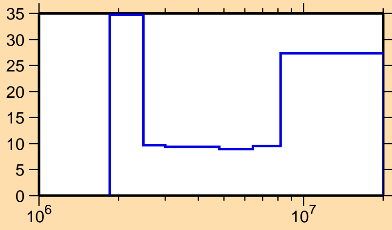
\Delta\sigma/\sigma vs. E for ^{91}\text{Y}(n,ncont.)
