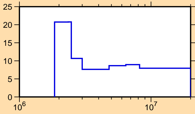
\Delta\sigma/\sigma vs. E for ^{91}\text{Y}(n,n\text{nonel.})
