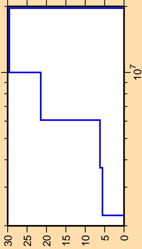
\Delta\sigma/\sigma vs. E for ^{92}\text{Y}(n,ncont.)
