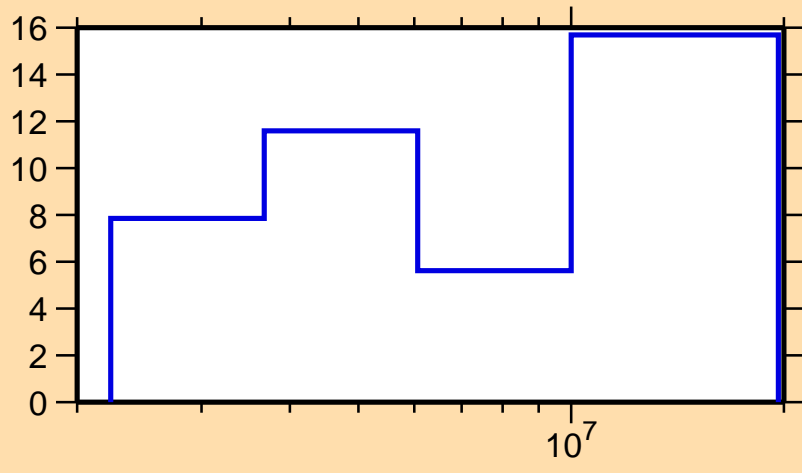
\Delta\sigma/\sigma vs. E for ^{92}\text{Y}(n,el.)
