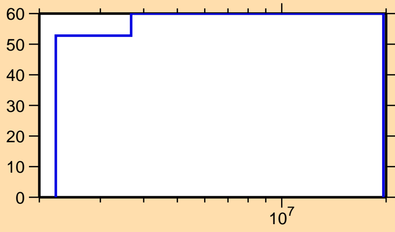
\Delta\sigma/\sigma vs. E for ^{92}\text{Y}(n,n_1)
