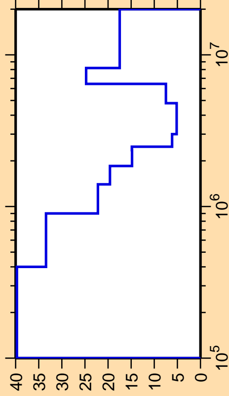
\Delta\sigma/\sigma vs. E for ^{92}\text{Y}(n,\text{inel.})
