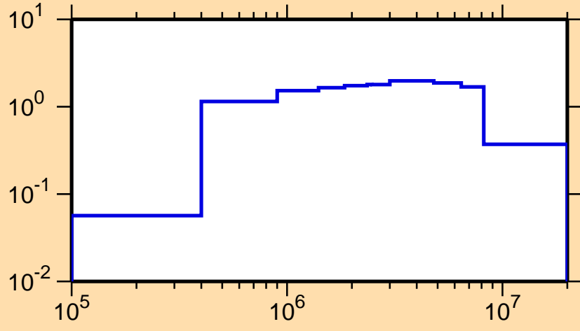
\sigma vs. E for ^{92}\text{Y}(n,\text{inel.})
