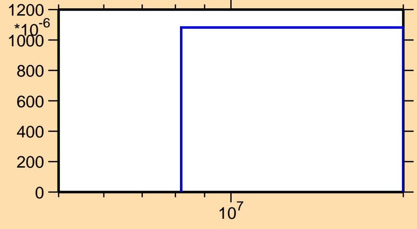
\sigma vs. E for ^{92}\text{Y}(n,np)
