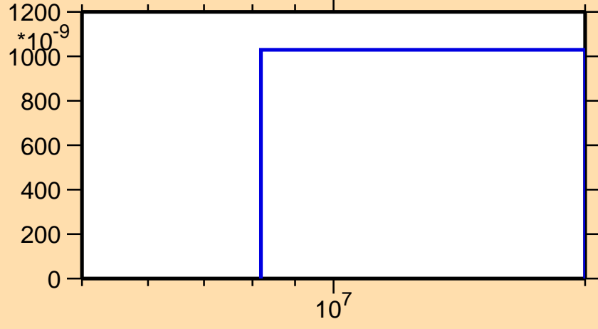
\sigma vs. E for ^{92}\text{Y}(n,\text{nd})
