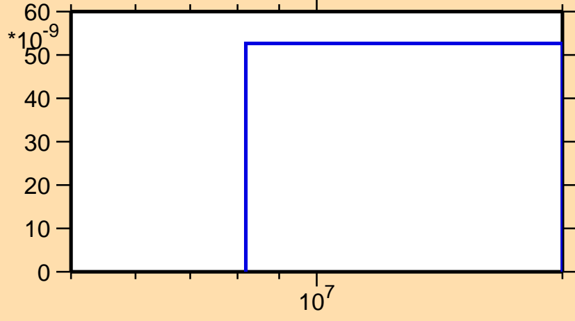
\sigma vs. E for ^{92}\text{Y}(n,nt)
