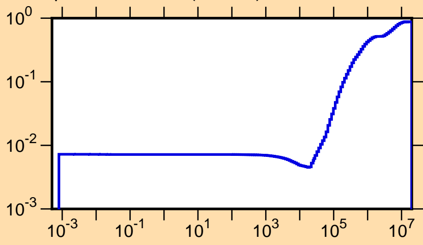
\mu vs. E for ^{93}\text{Y}(\text{mt251})
