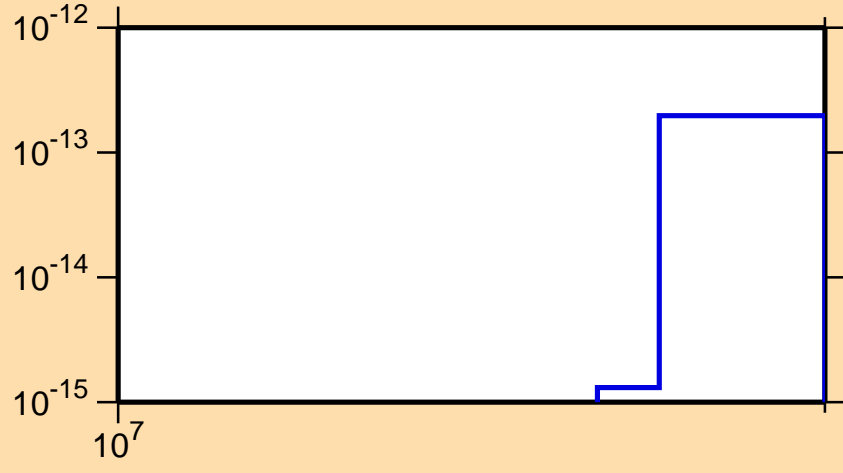
\sigma vs. E for ^{93}\text{Y}(n,p\alpha)
