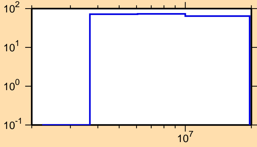
\Delta\sigma/\sigma vs. E for ^{93}\text{Y}(n,p)
