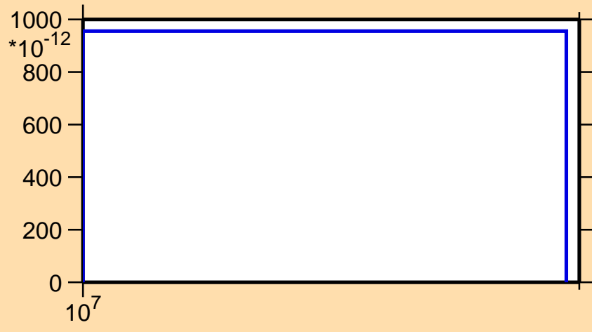
\sigma vs. E for ^{93}\text{Y}(n,2np)
