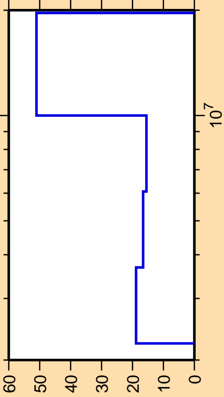
\Delta\sigma/\sigma vs. E for ^{93}\text{Y}(n,n\text{cont.})
