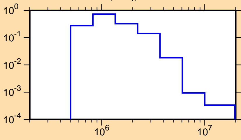
\sigma vs. E for ^{93}\text{Y}(n,n_1)
