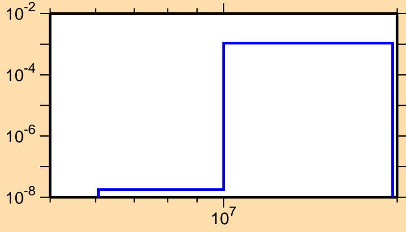
\sigma vs. E for ^{93}\text{Y}(n,d)
