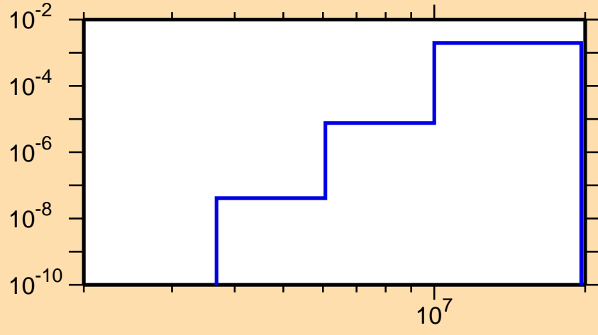
\sigma vs. E for ^{93}\text{Y}(n,\alpha)
