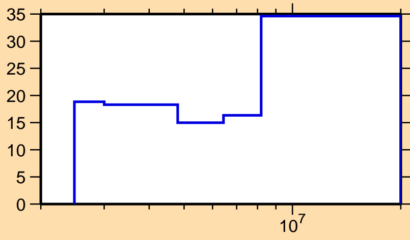
\Delta\sigma/\sigma vs. E for ^{93}\text{Y}(n,n\text{cont.})
