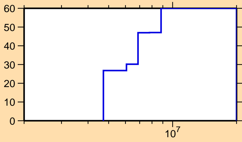
\Delta\sigma/\sigma vs. E for ^{94}\text{Y}(n,n\text{cont.})
