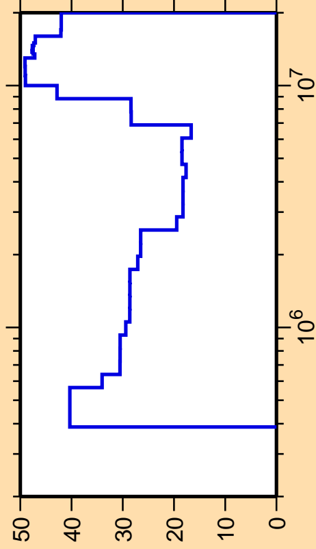
\Delta\sigma/\sigma vs. E for ^{94}\text{Y}(n,\text{inel.})
