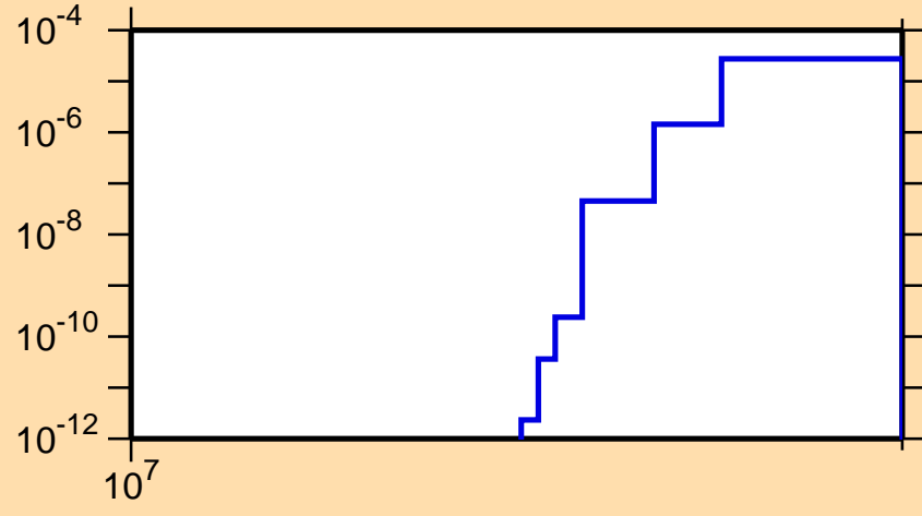
\sigma vs. E for ^{94}\text{Y}(n,nd)
