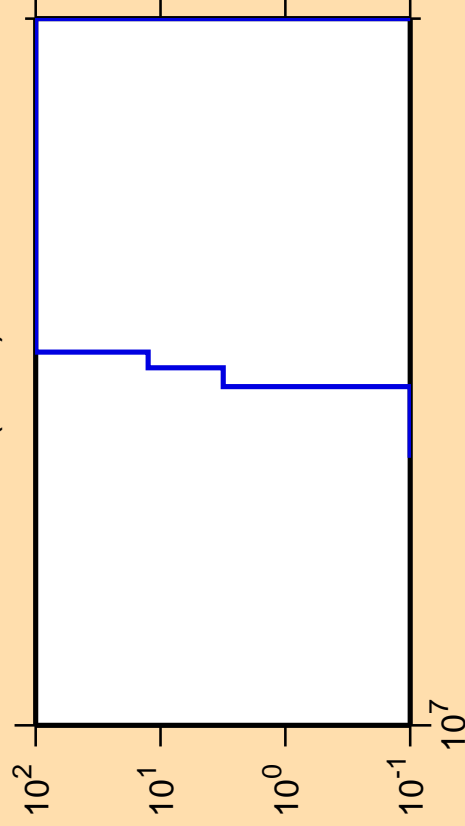
\Delta\sigma/\sigma vs. E for ^{94}\text{Y}(n,nd)
