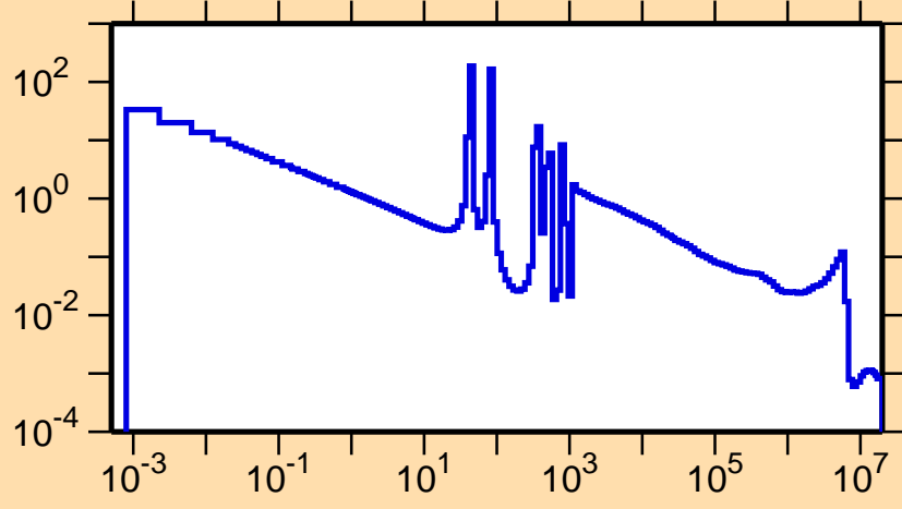
\sigma vs. E for ^{94}\text{Y}(n,\gamma)
