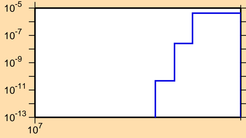
\sigma vs. E for ^{94}\text{Y}(n,nt)
