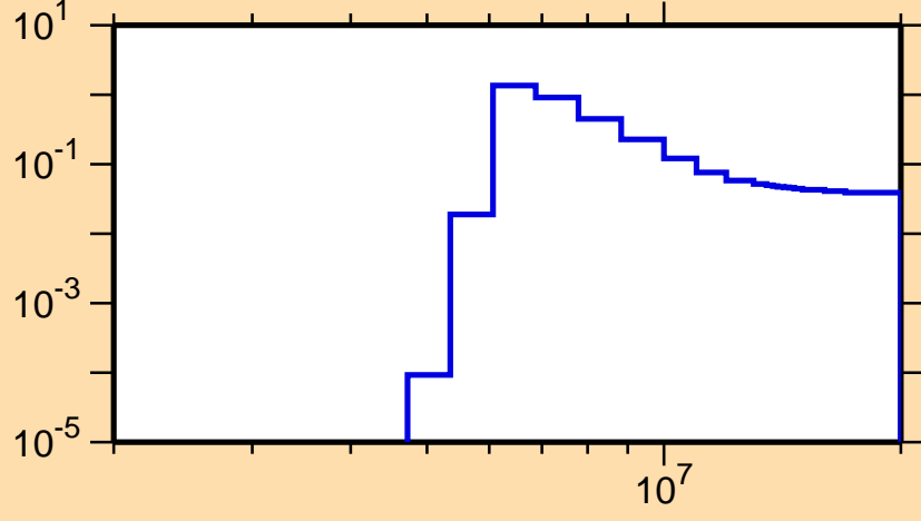
\sigma vs. E for ^{94}\text{Y}(n,n\text{cont.})
