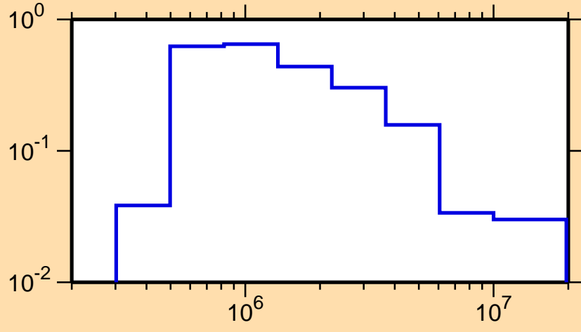
\sigma vs. E for ^{94}\text{Y}(n,n_1)
