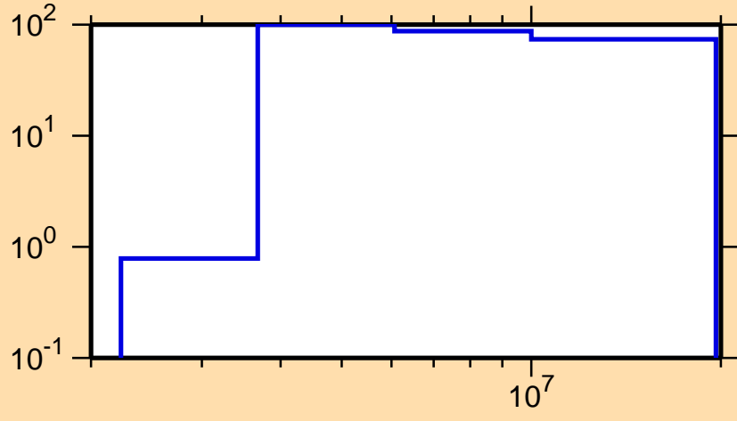
\Delta\sigma/\sigma vs. E for ^{94}\text{Y}(n,p)
