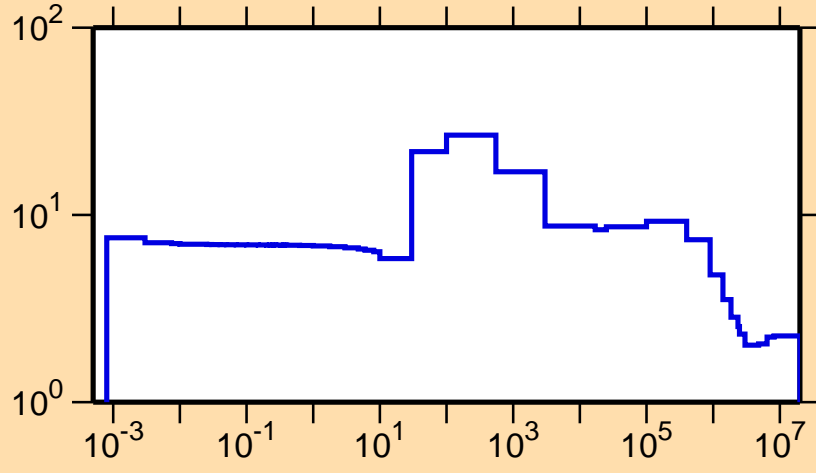
\sigma vs. E for ^{94}\text{Y}(n,\text{el.})
