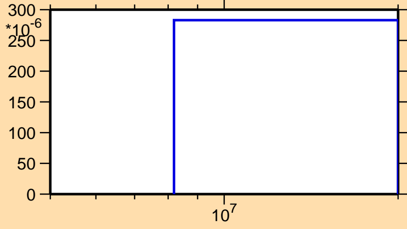
\sigma vs. E for ^{94}\text{Y}(n,np)
