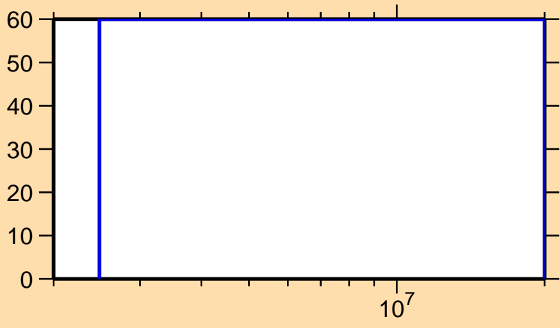
\Delta\sigma/\sigma vs. E for ^{94}\text{Y}(n,\gamma)
