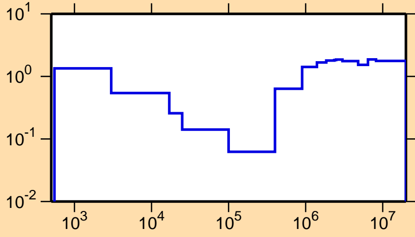
\sigma vs. E for ^{94}\text{Y}(n,\text{nonel.})
