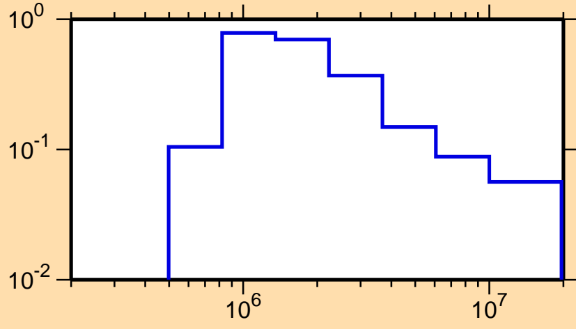
\sigma vs. E for ^{95}\text{Y}(n,n_1)
