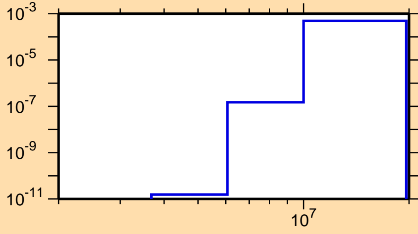
\sigma vs. E for ^{95}\text{Y}(n,\alpha)
