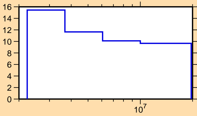
\Delta\sigma/\sigma vs. E for ^{95}\text{Y}(n,n\text{onel.})
