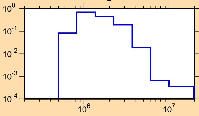
\sigma vs. E for ^{97}\text{Y}(n,n_2)
