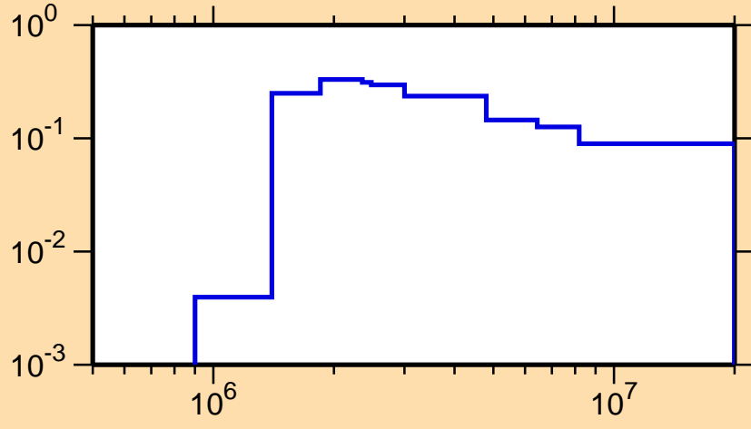
\sigma vs. E for ^{97}\text{Y}(n,n_4)
