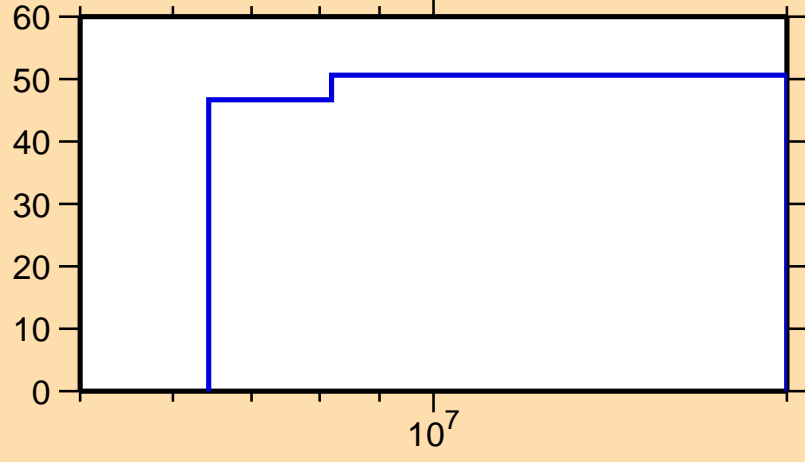
\Delta\sigma/\sigma vs. E for ^{97}\text{Y}(n,n_1)
