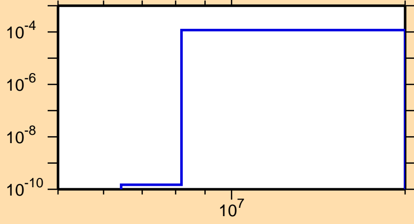
\sigma vs. E for ^{97}\text{Y}(n,\alpha)
