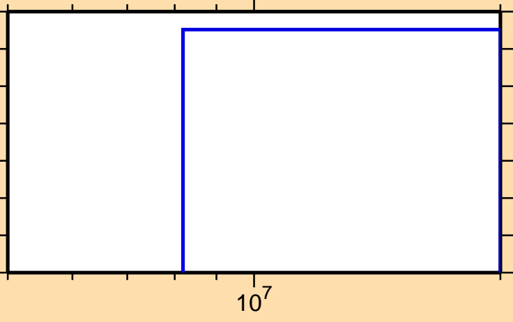
\sigma vs. E for ^{97}\text{Y}(n,\text{nd})
