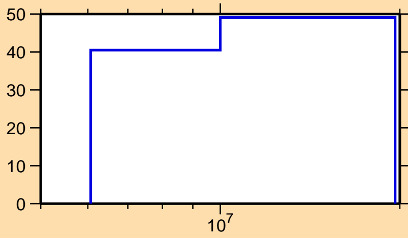
\Delta\sigma/\sigma vs. E for ^{97}\text{Y}(n,ncont.)
