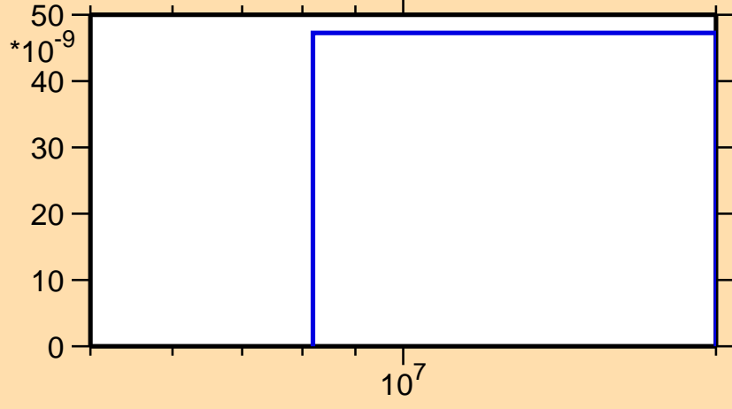
\sigma vs. E for ^{97}\text{Y}(n,\text{nd})
