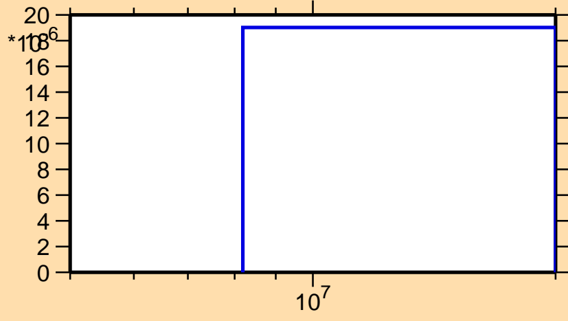
\sigma vs. E for ^{97}\text{Y}(n,n\alpha)
