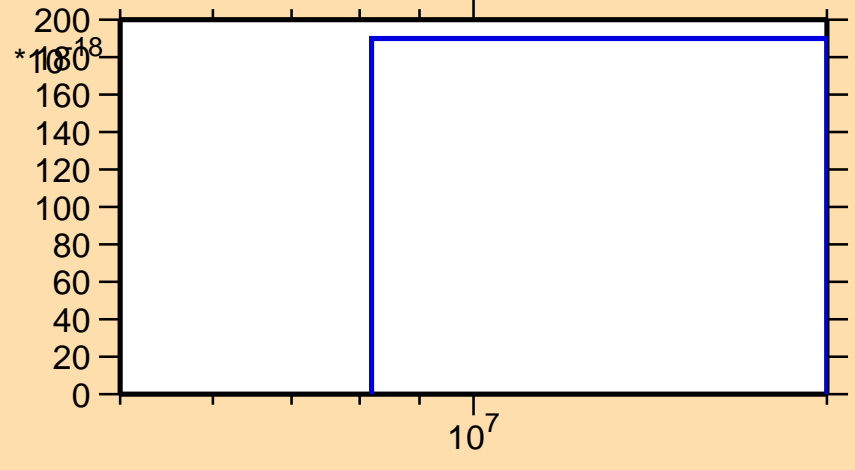
\sigma vs. E for ^{97}\text{Y}(\text{mt } 11)
