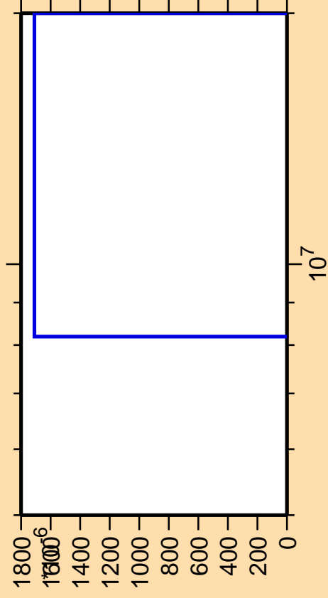
\Delta\sigma/\sigma vs. E for ^{97}\text{Y}(\text{mt } 11)
