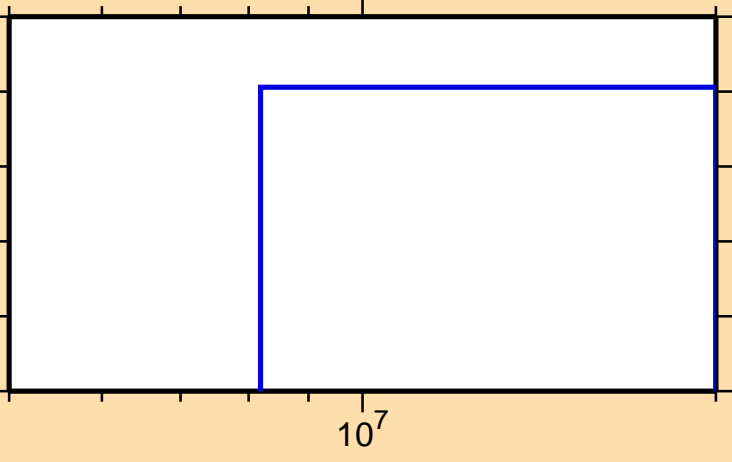
\sigma vs. E for ^{97}\text{Y}(n,nt)
