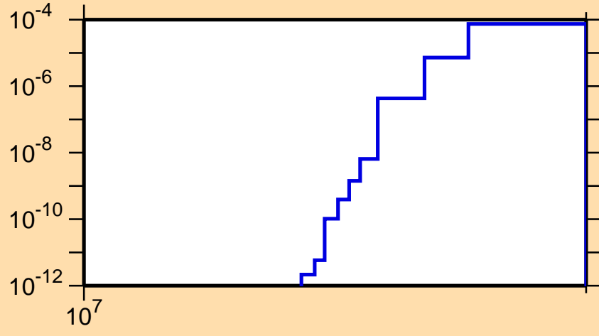
\sigma vs. E for ^{98}\text{Y}(n,nt)
