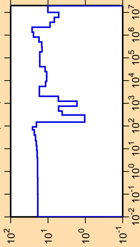
\Delta\sigma/\sigma vs. E for ^{98}\text{Y}(n,\text{el.})
