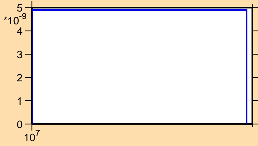
\sigma vs. E for ^{98}\text{Y}(n,2n\alpha)
