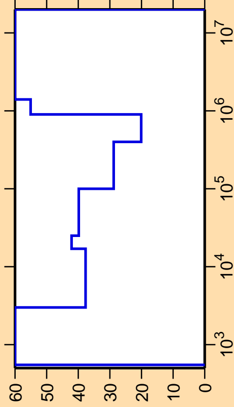
\Delta\sigma/\sigma vs. E for ^{98}\text{Y}(n,n_1)
