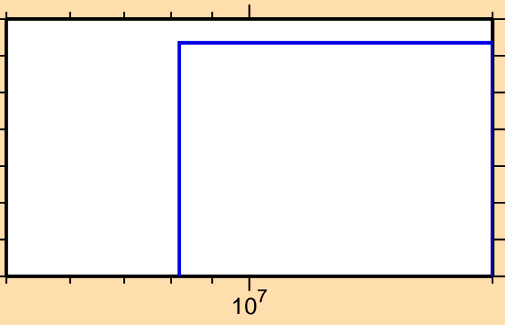
\sigma vs. E for ^{98}\text{Y}(n,n\alpha)
