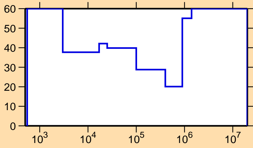
\Delta\sigma/\sigma vs. E for ^{98}\text{Y}(n,n_1)
