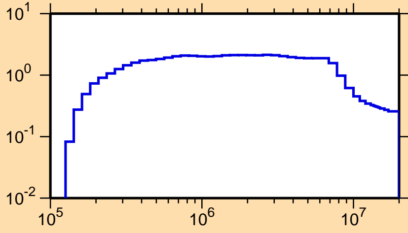
\sigma vs. E for ^{99}\text{Y}(n,\text{inel.})
