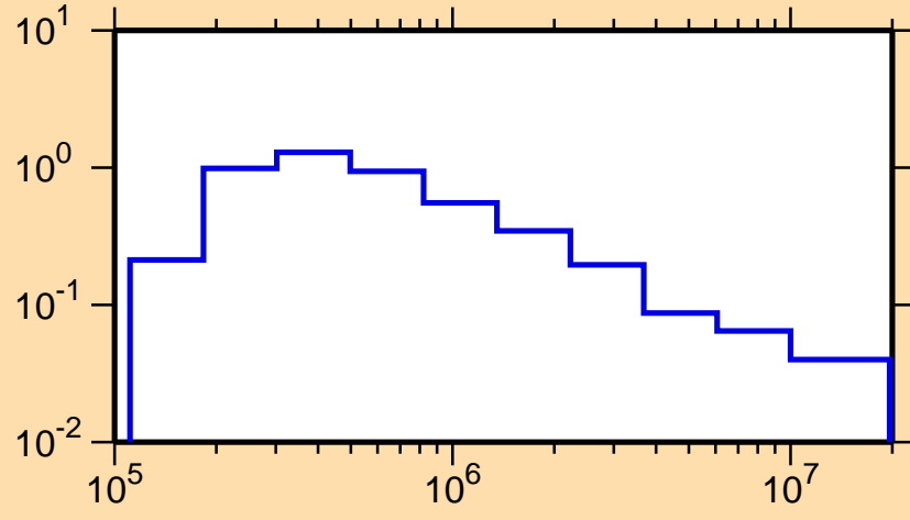
\sigma vs. E for ^{99}\text{Y}(n,n_1)
