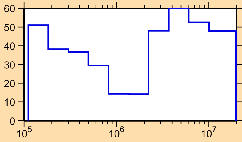
\Delta\sigma/\sigma vs. E for ^{99}\text{Y}(n,n_1)
