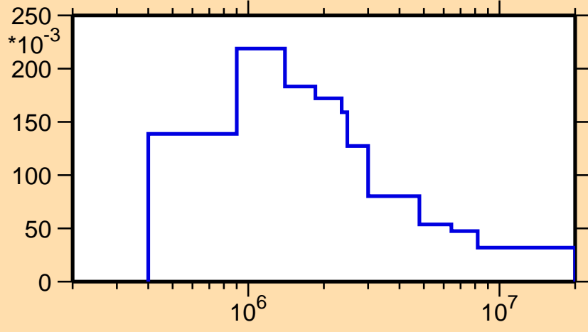
\sigma vs. E for ^{99}\text{Y}(n,n_4)
