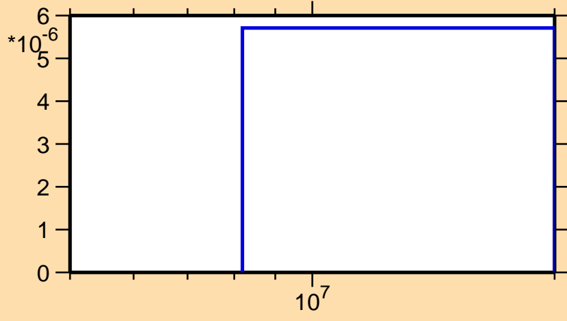
\sigma vs. E for ^{99}\text{Y}(n,t)
