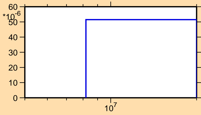
\sigma vs. E for ^{99}\text{Y}(n,d)
