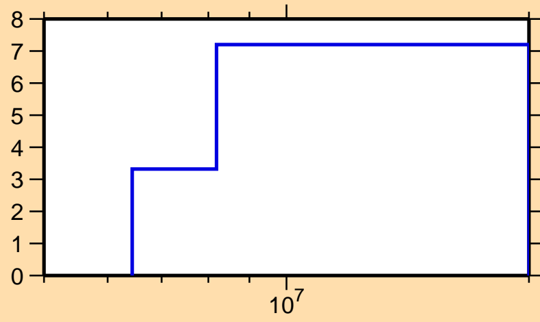
\Delta\sigma/\sigma vs. E for ^{99}\text{Y}(n,\text{tot.})
