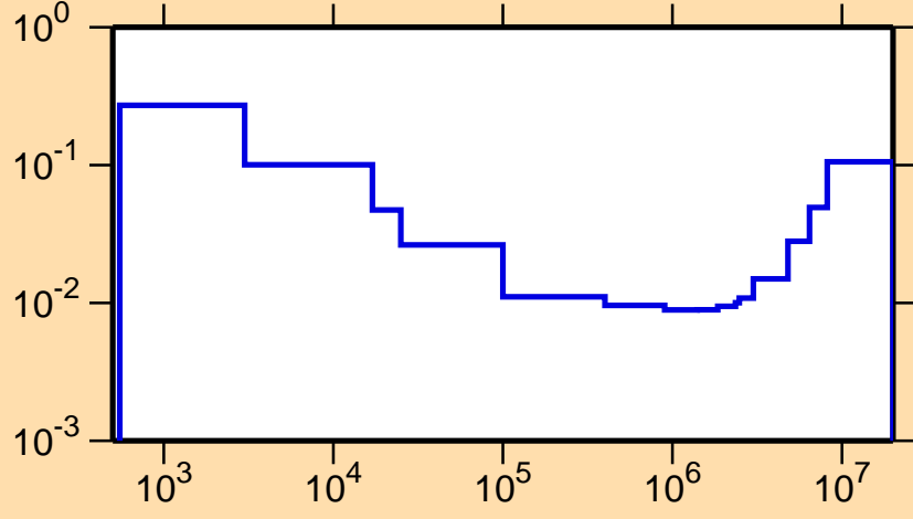
\sigma vs. E for ^{151}\text{Yb}(n,\alpha)
