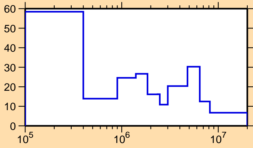
\Delta\sigma/\sigma vs. E for ^{151}\text{Yb}(n, el.)
