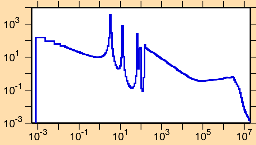
\sigma vs. E for ^{152}\text{Yb}(n,\gamma)
