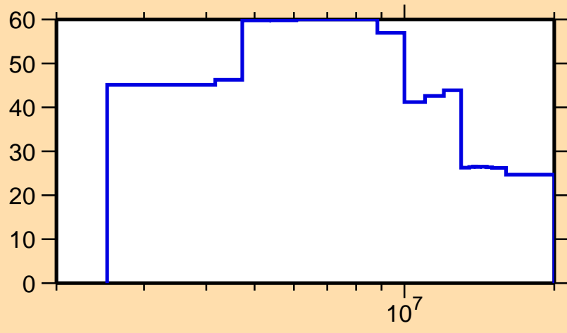
\Delta\sigma/\sigma vs. E for ^{152}\text{Yb}(n,n\text{cont.})
