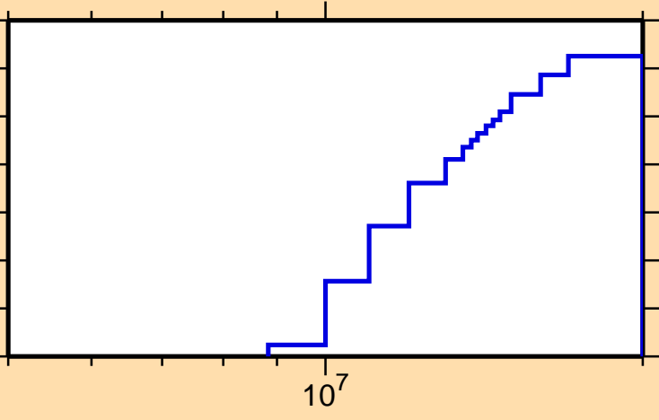
\sigma vs. E for ^{152}\text{Yb}(\text{mt117})
