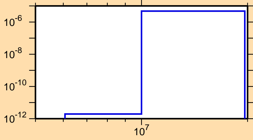
\sigma vs. E for ^{152}\text{Yb}(\text{mt } 45)
