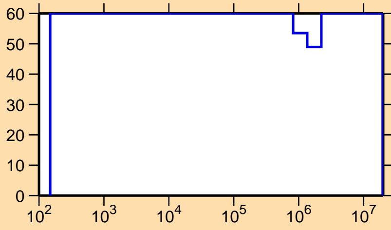
\Delta\sigma/\sigma vs. E for ^{152}\text{Yb}(n,\gamma)
