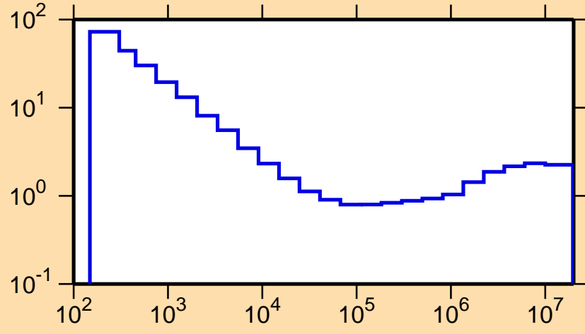
\sigma vs. E for ^{152}\text{Yb}(n,\text{nonel.})
