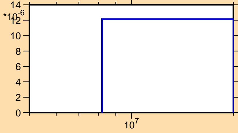
\sigma vs. E for ^{152}\text{Yb}(n,t)
