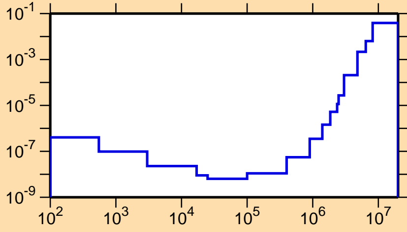
\sigma vs. E for ^{152}\text{Yb}(n,p\alpha)
