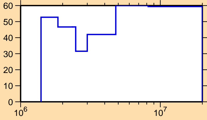
\Delta\sigma/\sigma vs. E for ^{152}\text{Yb}(n,n_1)
