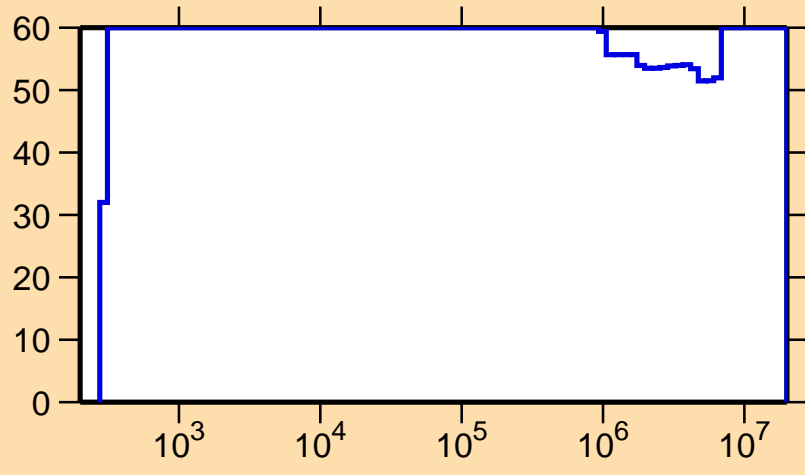
\Delta\sigma/\sigma vs. E for ^{153}\text{Yb}(n,\gamma)
