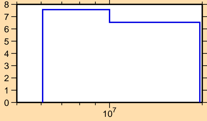
\Delta\sigma/\sigma vs. E for ^{153}\text{Yb}(n,\text{nonel.})
