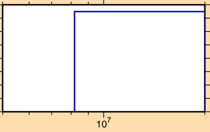
\sigma vs. E for ^{153}\text{Yb}(n,\text{pt})
