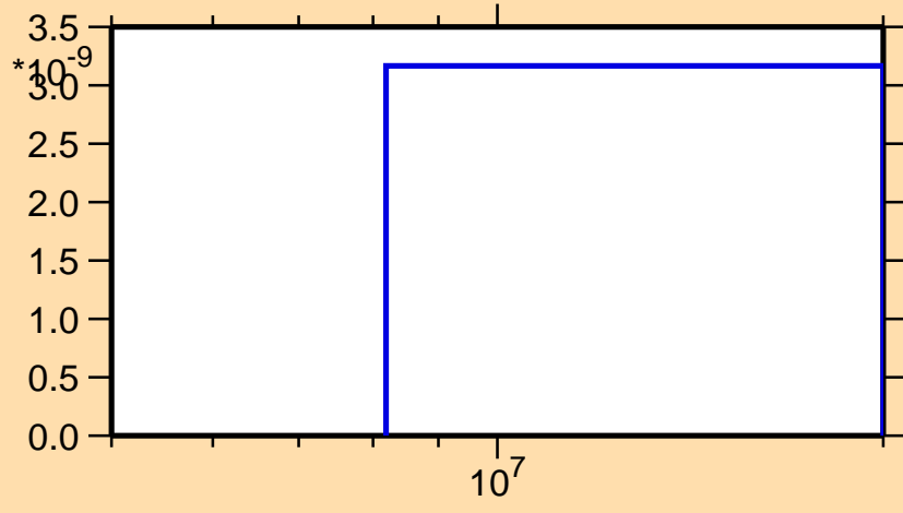
\sigma vs. E for ^{153}\text{Yb} (mt 34)
