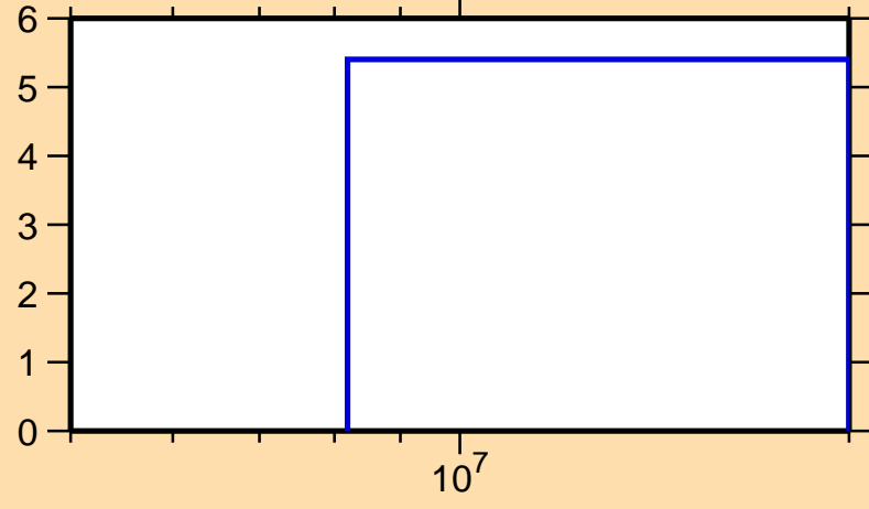
\Delta\sigma/\sigma vs. E for ^{153}\text{Yb}(n,\text{el.})
